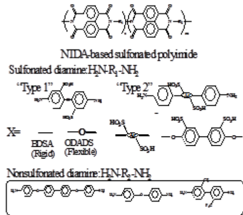
Fig.1 Chemical structures of sulfonated polyimides
